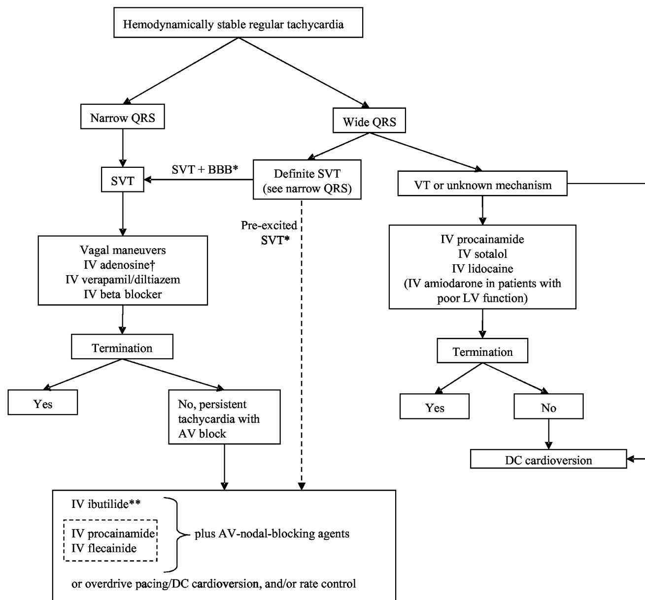
Figure 7. Acute management of patients with hemodynamically stable and regular tachycardia. *A 12-lead ECG during sinus rhythm must be available for diagnosis. †Adenosine should be used with caution in patients with severe coronary artery disease and may produce AF, which may result in rapid ventricular rates for patients with pre-excitation. **Ibutilide is especially effective for patients with atrial flutter but should not be used in patients with EF less than 30% due to increased risk of polymorphic VT. AF indicates atrial fibrillation; AV, atrioventricular; BBB, bundle-branch block; DC, direct current; IV, intravenous; LV, left ventricle; QRS, ventricular activation on ECG; SVT, supraventricular tachycardia; VT, ventricular tachycardia.
