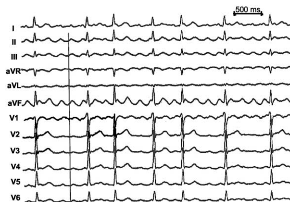
Figure 11. 12-Lead ECG from a patient with clockwise cavotricuspid isthmus-dependent flutter. Note that the flutter waves are positive in the inferior leads and predominantly negative double waves in lead V1. ms indicates milliseconds.
