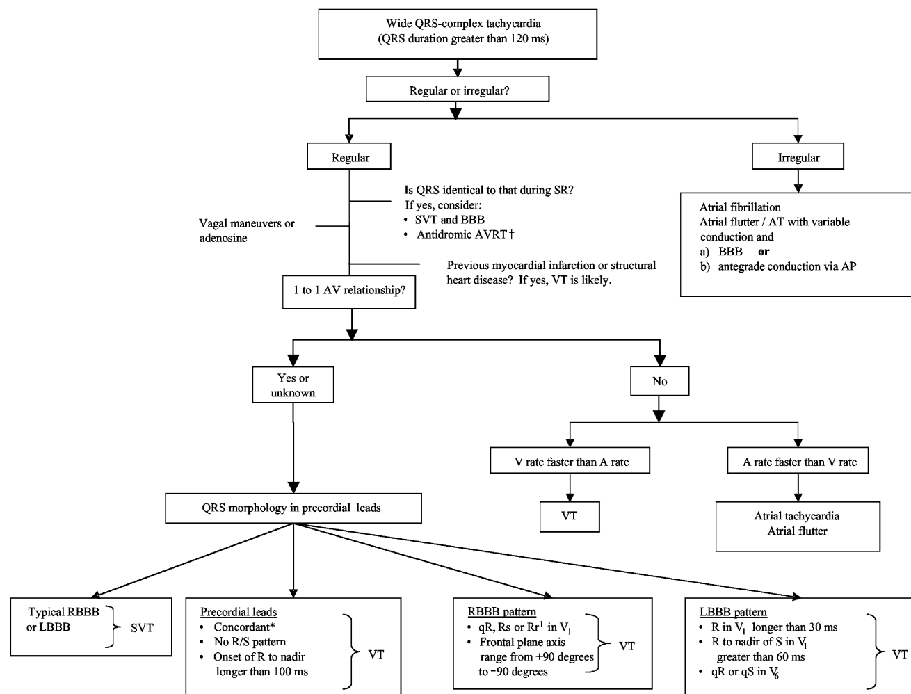
Figure 5. Differential diagnosis for wide QRS-complex tachycardia (more than 120 ms). A QRS conduction delay during sinus rhythm, when available for comparison, reduces the value of QRS morphology analysis. Adenosine should be used with caution when the diagnosis is unclear because it may produce VF in patients with coronary artery disease and AF with a rapid ventricular rate in pre-excited tachycardias. Various adenosine responses are shown in Figure 4. *Concordant indicates that all precordial leads show either positive or negative deflections. Fusion complexes are diagnostic of VT. †In pre-excited tachycardias, the QRS is generally wider (ie, more pre-excited) compared with sinus rhythm. A indicates atrial; AP, accessory pathway; AT, atrial tachycardia; AV, atrioventricular; AVRT, atrio-ventricular reciprocating tachycardia; BBB, bundle-branch block; LBBB, left bundle-branch block; ms, milliseconds; QRS, ventricular activation on ECG; RBBB, right bundle-branch block; SR, sinus rhythm; SVT, supraventricular tachycardias; V, ventricular; VF, ventricular fibrillation; VT, ventricular tachycardia.
